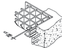
2" grating: PN# 6179000 Install 2" side vertical
