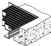
3" grating: PN# 6180005 Install 3" side vertical
