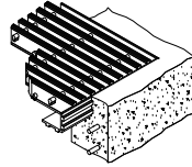
2-1/2" grating: PN# 6180005 Install 2-1/2" side vertical
