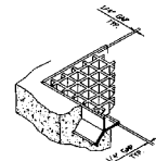
2" grating: PN# 6179000 Install 2" side vertical
