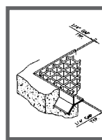
1" grating: PN# 6179100 Install 1" side vertical
